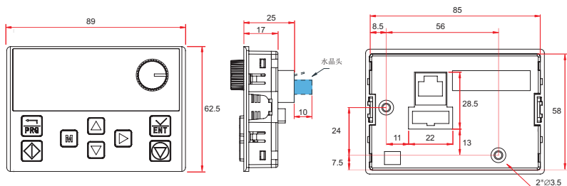
图8-14 ××××-JP-LED-BD外引+本机操作面板尺寸
